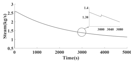
Fig. 13. Dynamic diagram of the heat supply during the internal combustion engine gas supply failure
