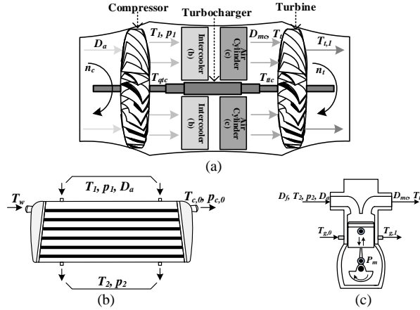
Fig. 2. Structural model diagram of gas engine. (a) Turbine compressor. (b) Intercooler. (c) Air cylinder.
