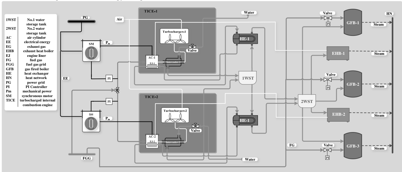
Fig. 1. Structure diagram of grid-connected combined heat and power system
