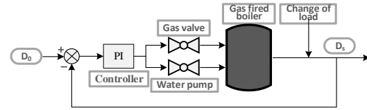
Fig. 7. Control flow chart of gas-fired boiler
